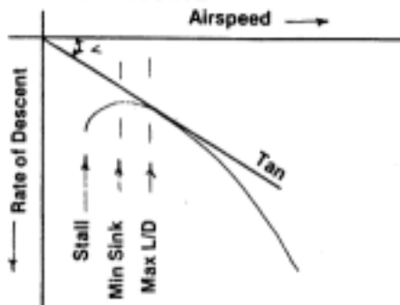
FIG. 2 POLAR CURVE
