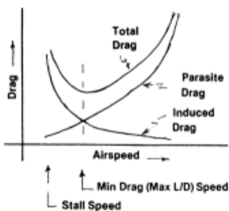
FIG. 1 DRAG CURVE
